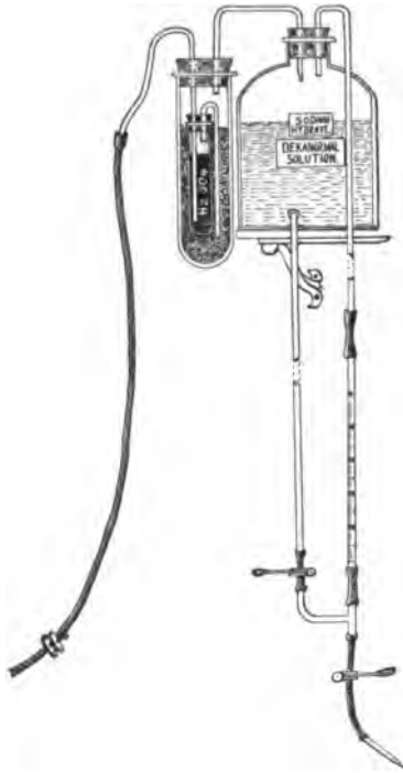
FIG. 99.—Stock bottle for deka-normal soda solution.
